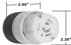
Corrosion-Resistant Connector
