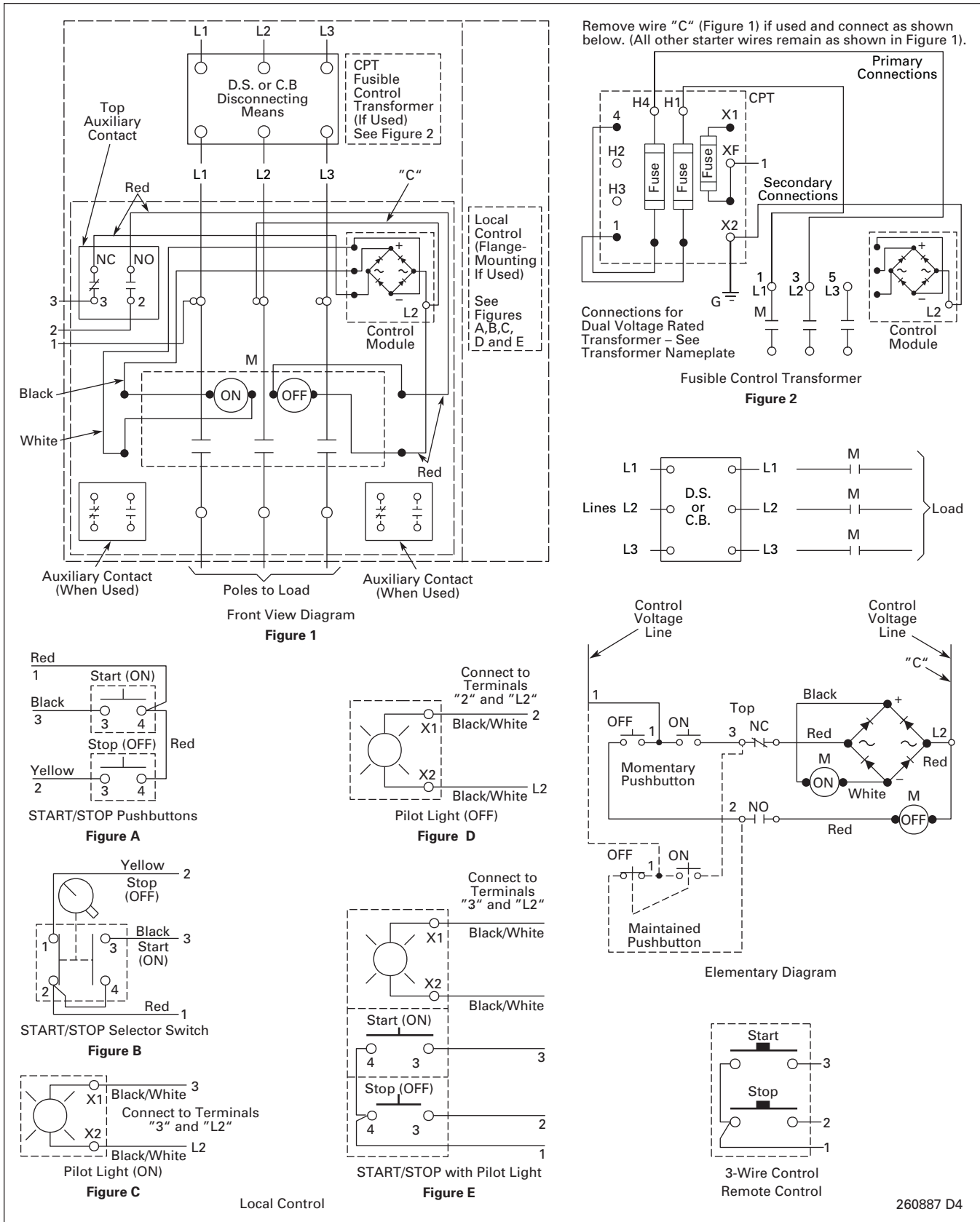
Figure 37-14. Magnetically Latched Combination Contactors
